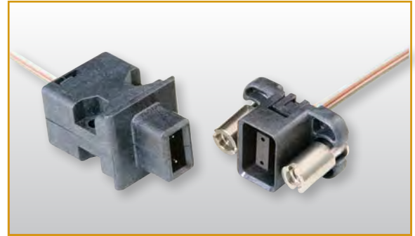
VME P0/J0 Connectors with MT ferrule fiber optics
