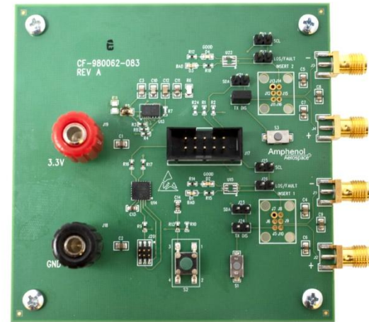
Test Board
