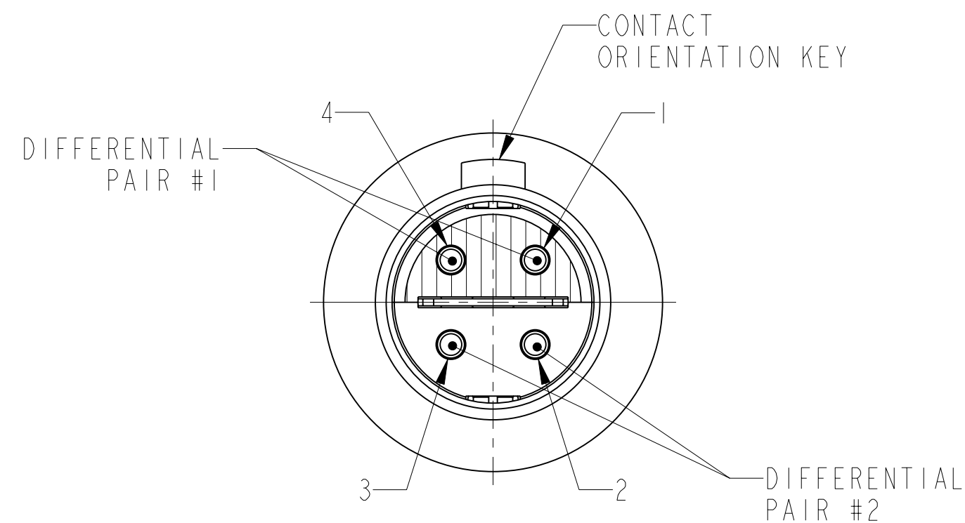
MATING FACE VIEW (RECOMMENDED CONTACT ID'S) SCALE 8:1
