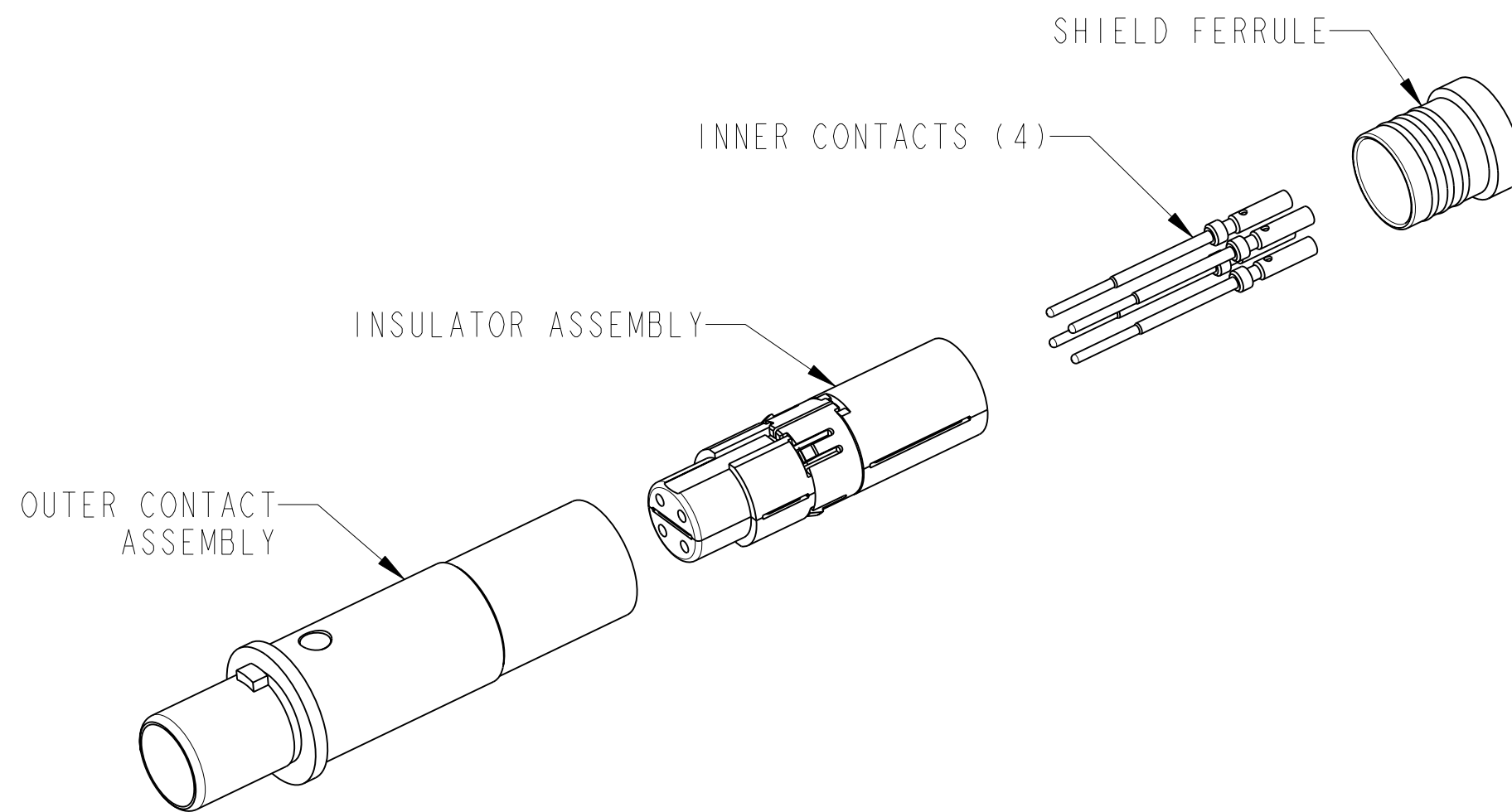
EXPLODED COMPONENT VIEW (PIGGYBACK SEAL NOT SHOWN) SCALE 3:1
