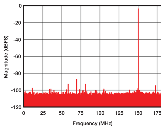
1 -Tone Spectrum, 150 MHz
