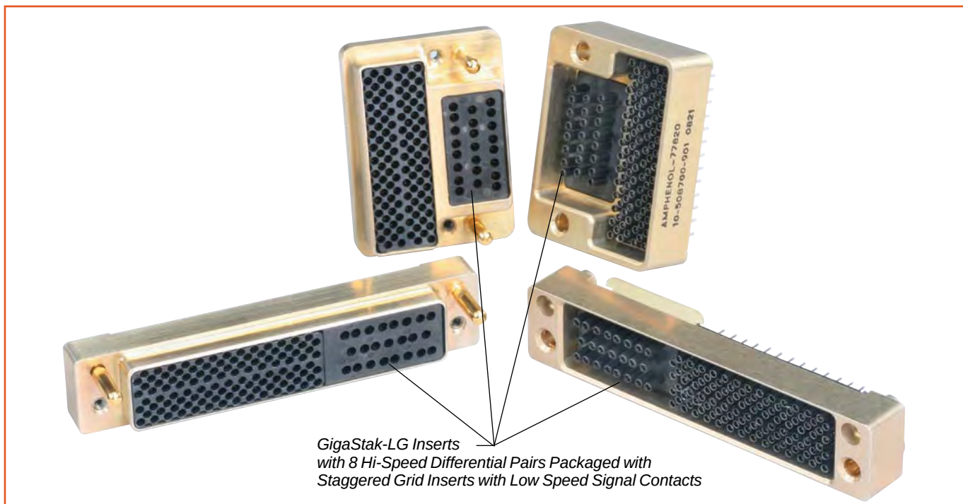
8 Differential Pairs and 108 Digital Contacts
