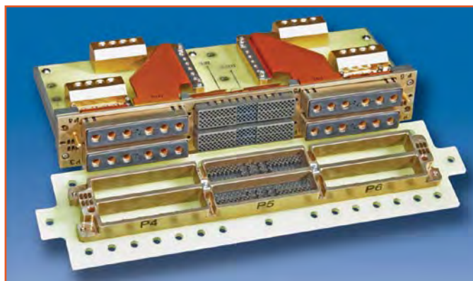
Flex circuitry used to attach to PC boards - designed to fit specific board requirements
