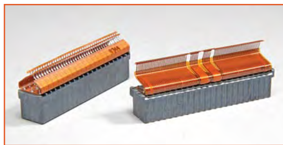
LRM module inserts with flex termination
