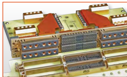
LRM special 6 bay design with RADSOK® contacts, standard brush contacts, and flex circuitry termination to module circuit card assemblies
