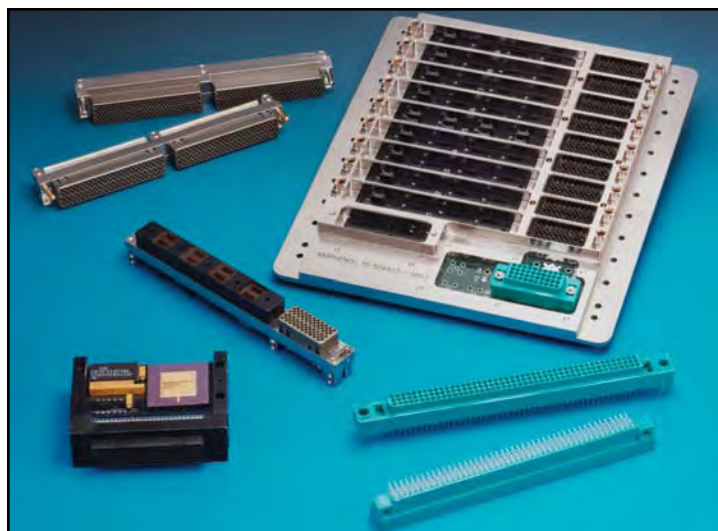
Amphenol rectangular products group, including low mating force PCB connectors, LRM connectors and the OBIS Backplane with brush contacts and MT ferrule fiber optics.
