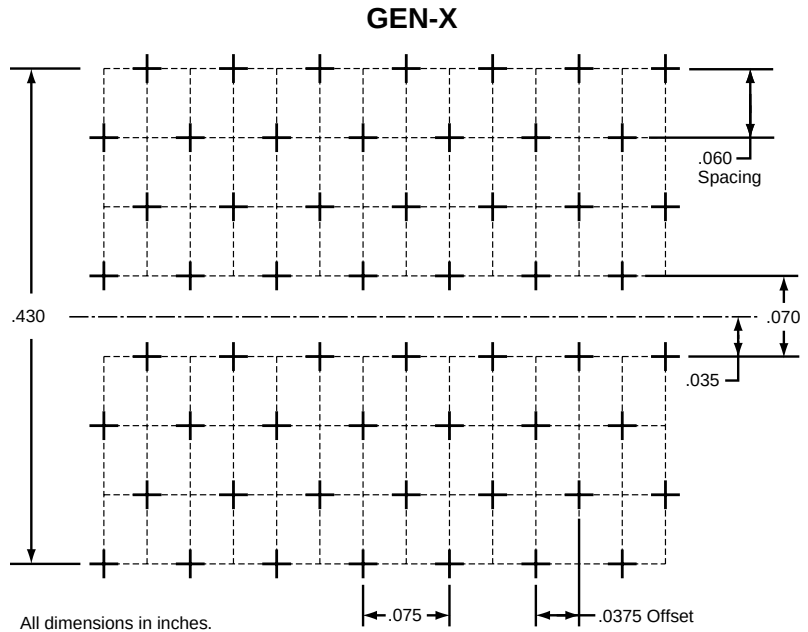
Example of a 3 bay GEN-X backplane connector.
