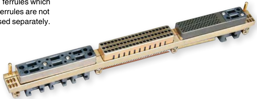
Example of an LRM module connector with MT fiber optic inserts in combination with inserts for brush LVDs and digital contacts.
