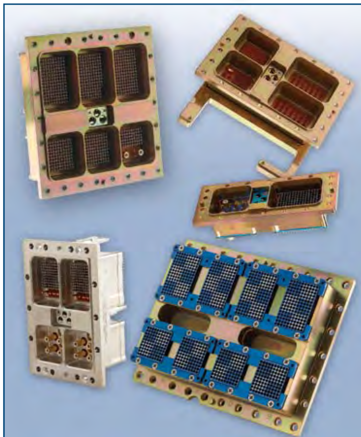
R27 Series Rack and Panel Connectors
