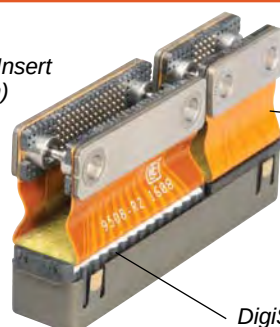
GigaStak-LG Inserts with 8 Hi-Speed Differential Pairs Packaged with Staggered Grid Inserts with Low Speed Signal Contacts
