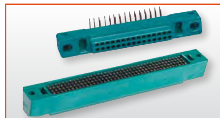
Low Mating Force Connectors - the first development of rectangulars with Brush contacts.
