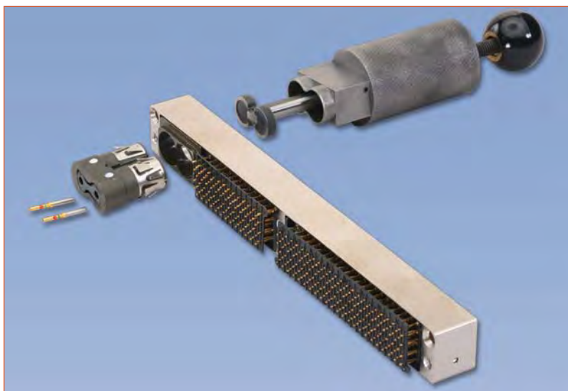
Exploded view - tool 10-507924-1 has removed power module from backplane. (Size 22D contacts shown removed)
