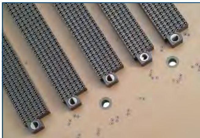
NAFI Backplane Connectors on Board
