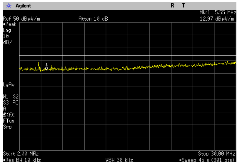
Plot 1.2: RE102 test results within 2 – 30 MHz, vertical polarization
