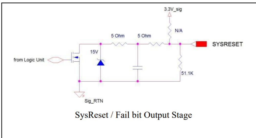
Figure 2 – SysRst and Fail Bit Output Stage
