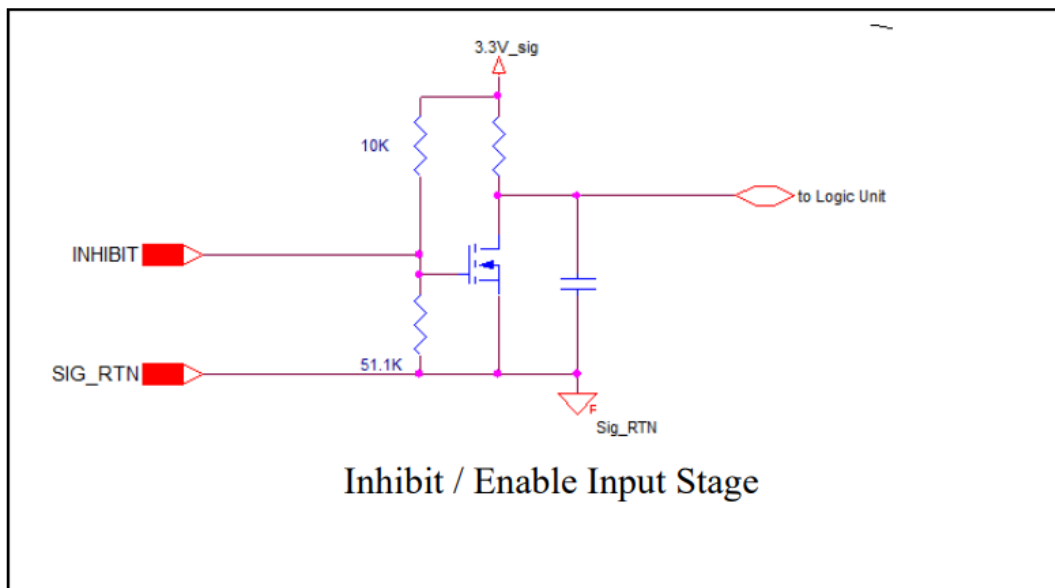
Figure 1 – Inhibit and Enable Input stage
