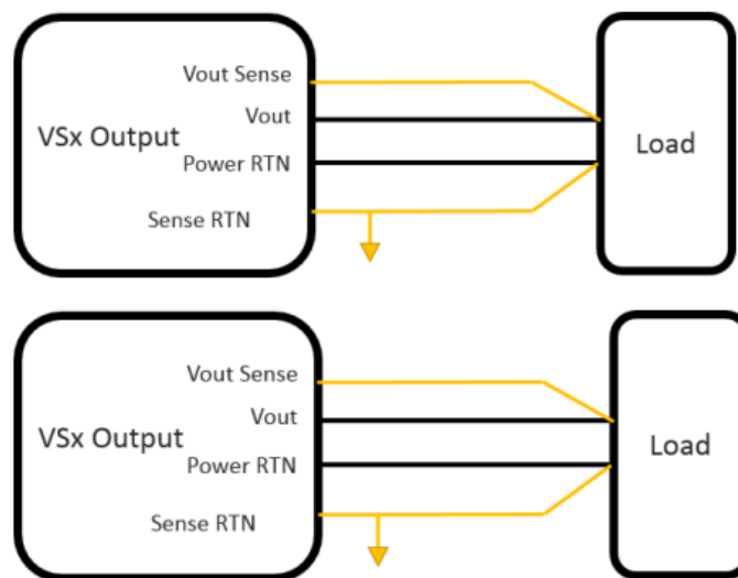
Figure 3: M4067 Sense line connection
