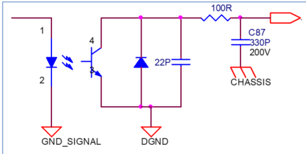
Figure 4 – Fault output interface
