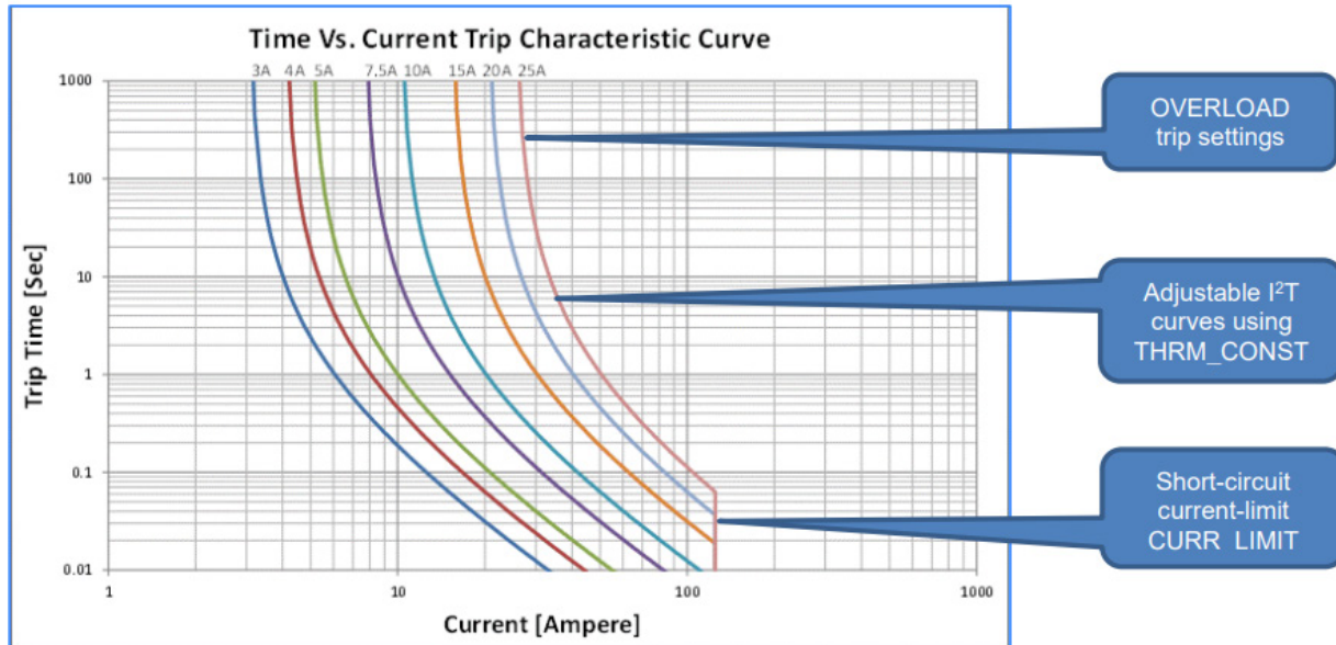
Figure 1 - Time vs. Current Overload Trip
