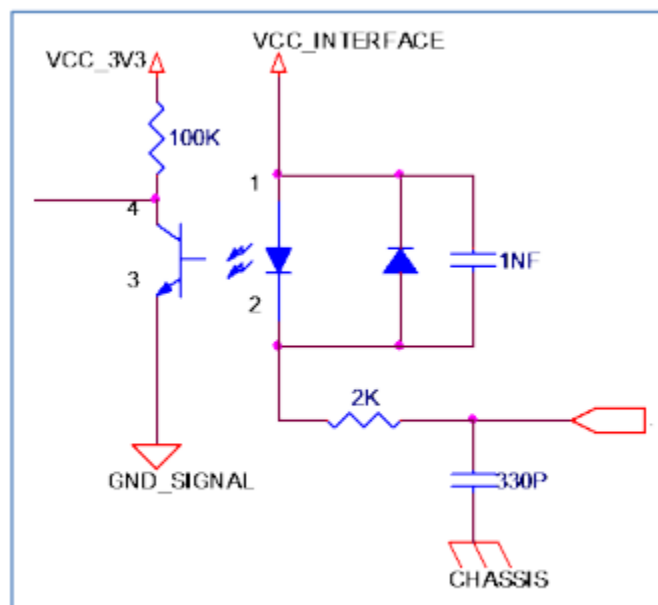
Figure 3 – Discrete input interface
