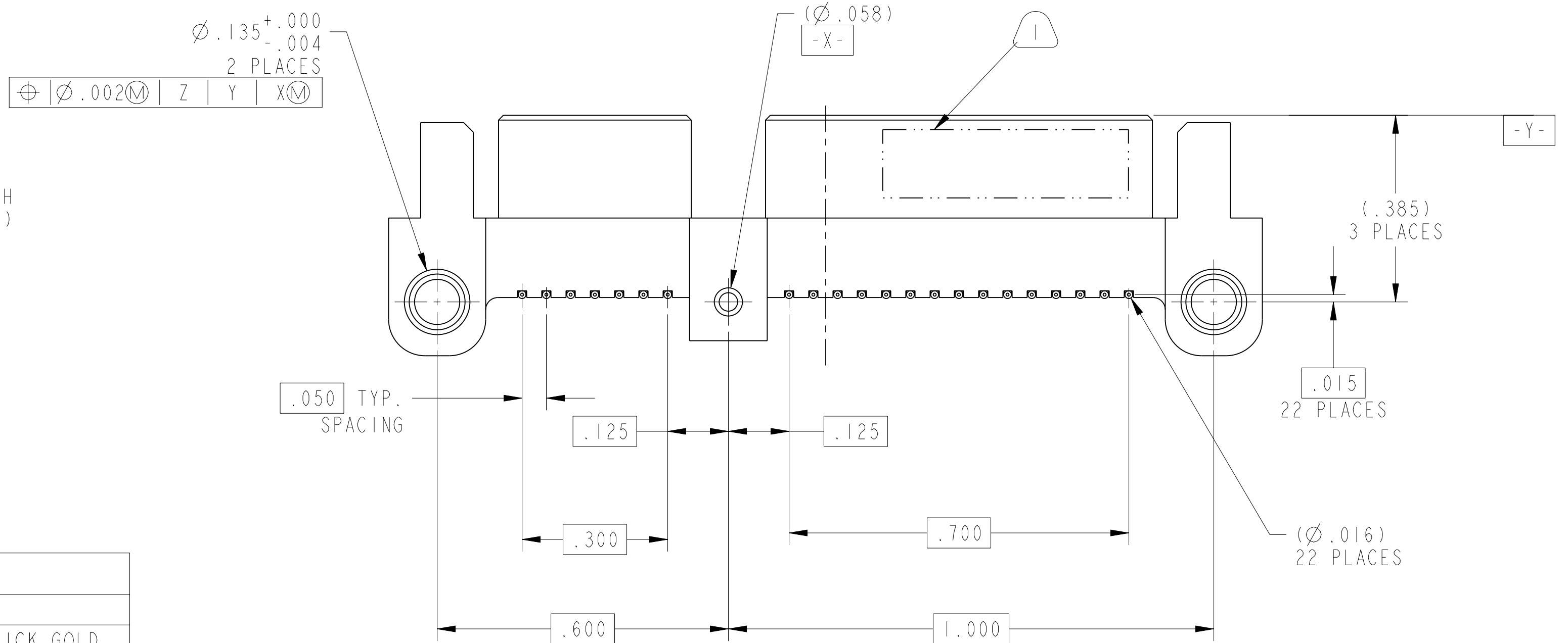
VIEW AT A
