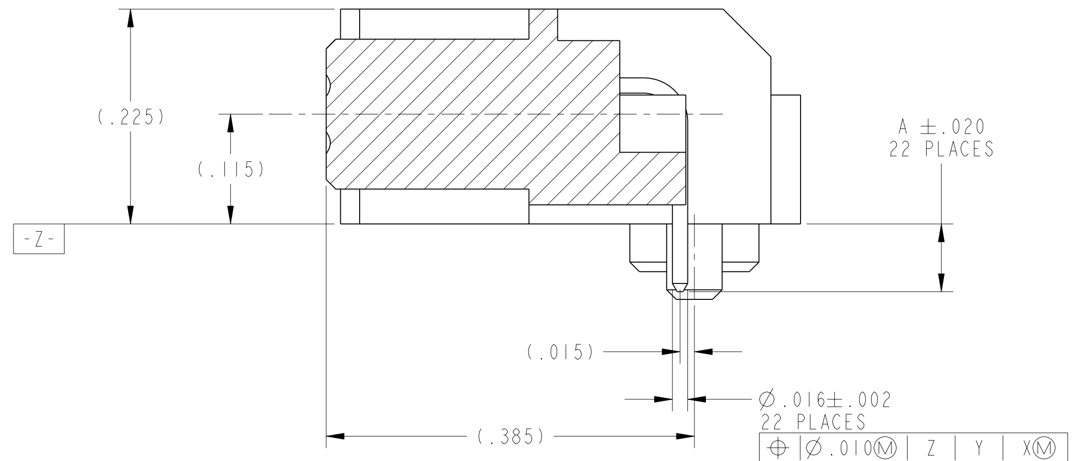
SECTION B-B
