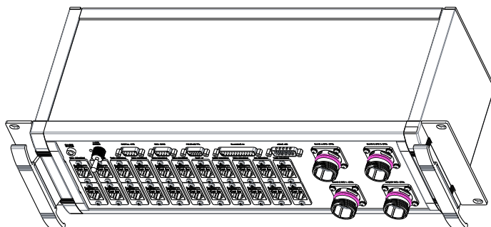
JUNCTION BOX ISO FRONT VIEW SCALE 0.500
