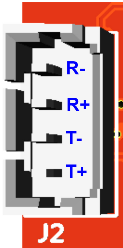
Figure 4: Ethernet port pinout
