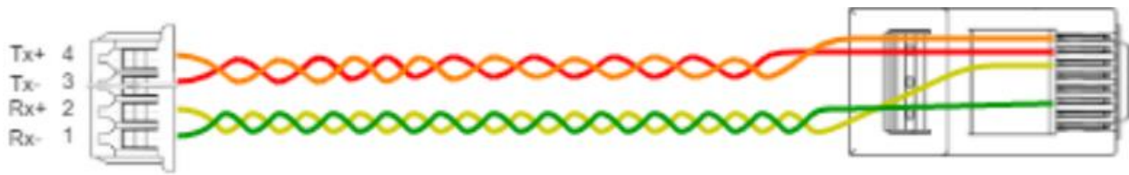
Ethernet cable pinout for Molex PicoBlade variant
