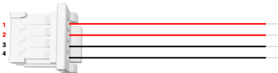
Voltage input cable pinout for Molex PicoClasp (red = V+, black = GND)
