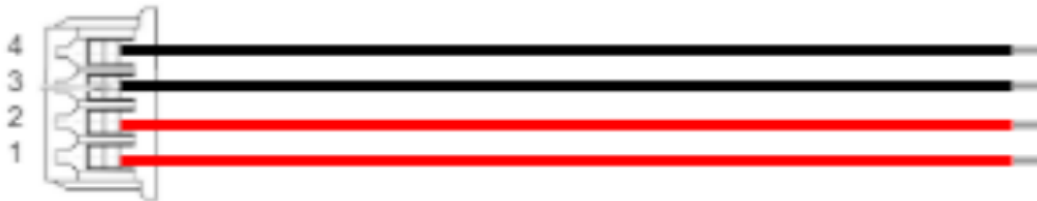
Voltage input cable pinout for Molex PicoBlade (red = V+, black = GND)
