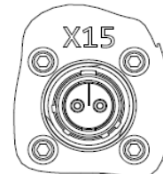
DETAIL F X1 THRU X18 CF-971912-02P SCALE 1.500
