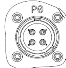
DETAIL C P0 POWER 10-646401-750N SCALE 1.500
