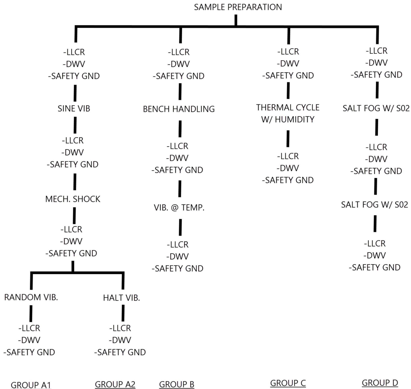
Figure 2: Test sequence groups A-D
