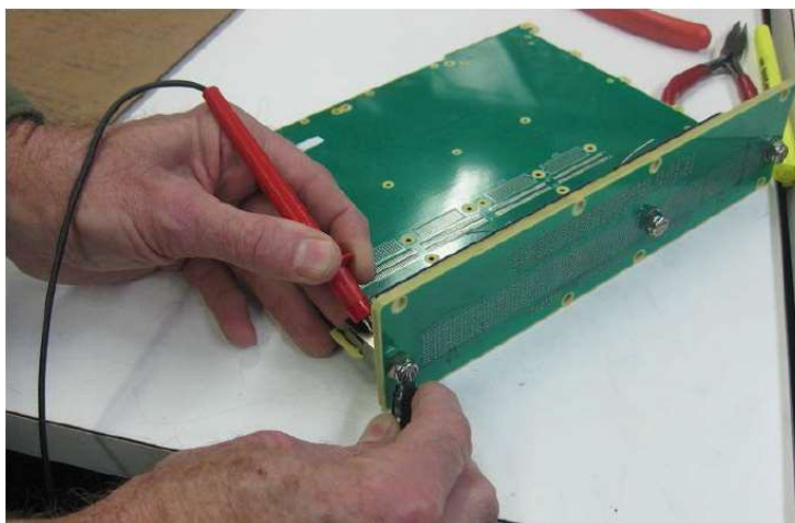
Figure 5: Typical Safety Ground Measurement set-up
