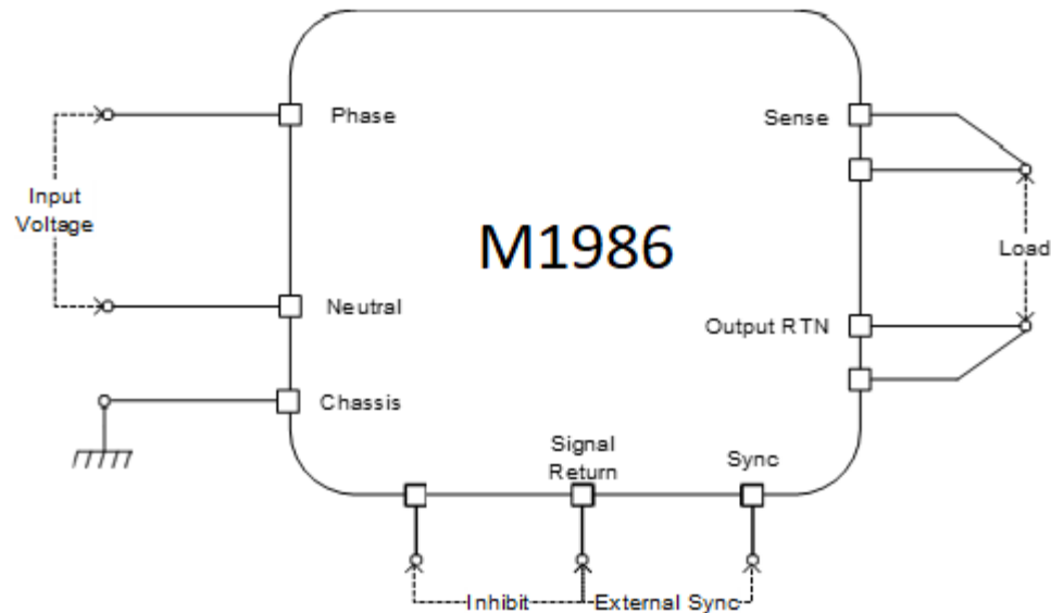
Typical Connection Diagram
