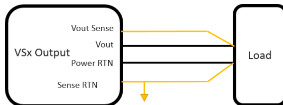
Figure 3: M4701 Sense line connection
