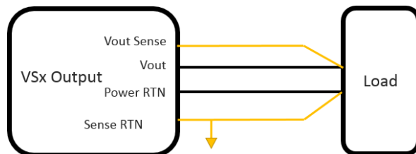
Figure 3 – Sense Lines connection
