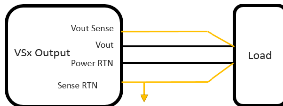
Figure 3: M4706 Sense line connection
