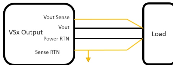
Figure 3: M4707 Sense line connection
