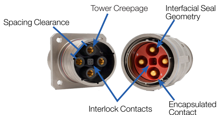
HIGH VOLTAGE 38999
