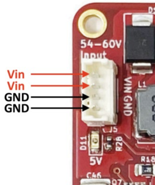
Voltage input header pinout
