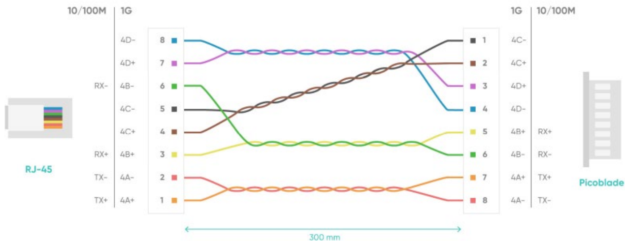
Ethernet cable pinout
