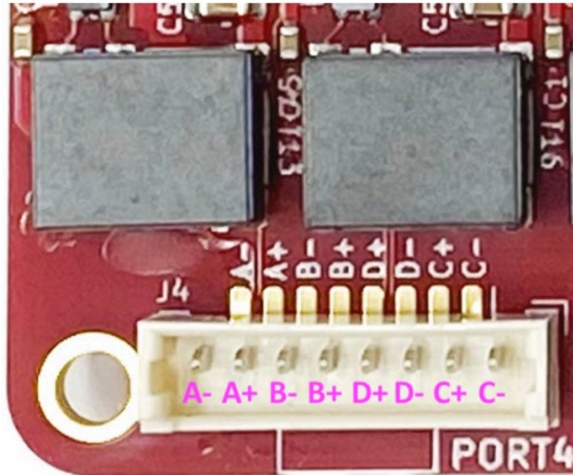
Ethernet pinout on Molex PicoBlade ports
