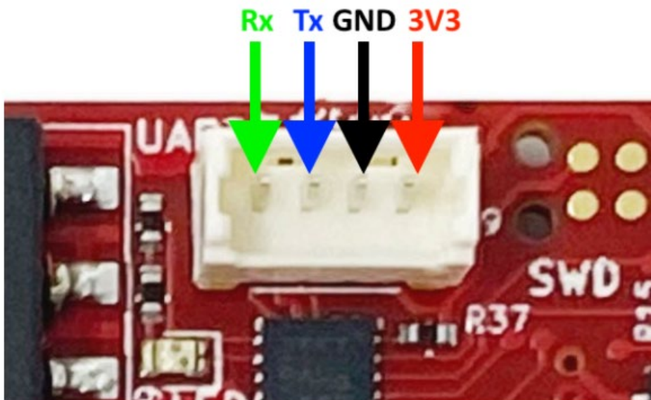
Pinout of the onboard UART port
