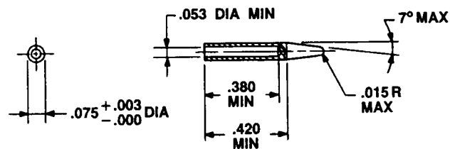
EXPANDER TOOL
